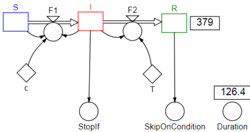
Figure 3. A stochastic SIR model in StochSD after a replication.
